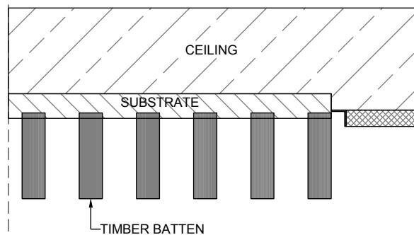
CEILING PANEL SHADOW TO ADJACENT GYPROCK CEILING WITH BEAM EXPOSED BELOW GYPROCK (P50 INTO SUBSTRATE EDGE)
