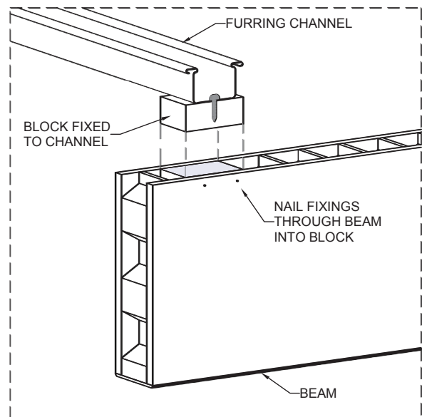
CARDBOARD CORE BEAMS
